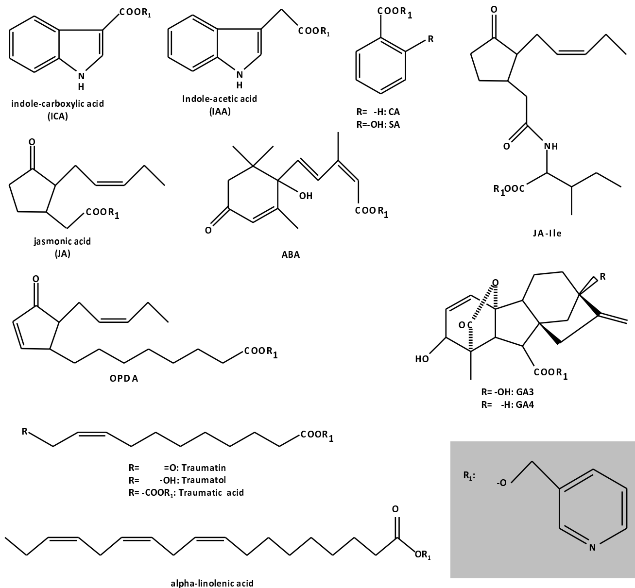
Figure 1 Examples of compounds analyzed as their Picolinyl ester derivatives by LC-MS/MS.
